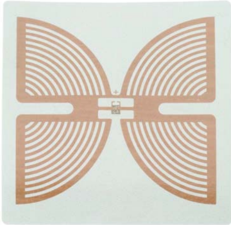
Figure 1: Class 1 tag insert (Butterfly style). Source: Courtesy of Intermec technologies
