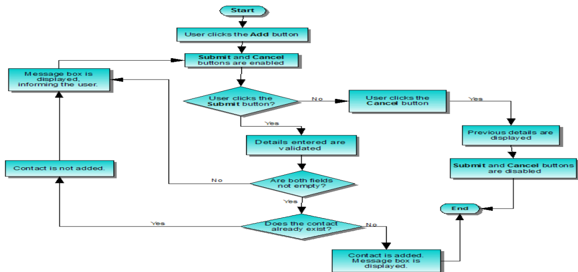
Figure 1.1: Developed Address Book Flowchart
