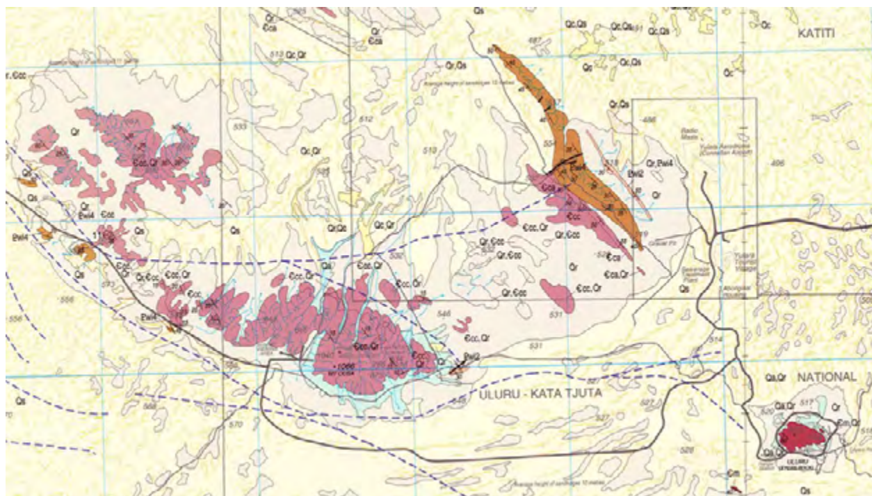
Figure 8: The geological map of Kata Tjuta and Uluru. Source: Australian Geoscience Information Network
